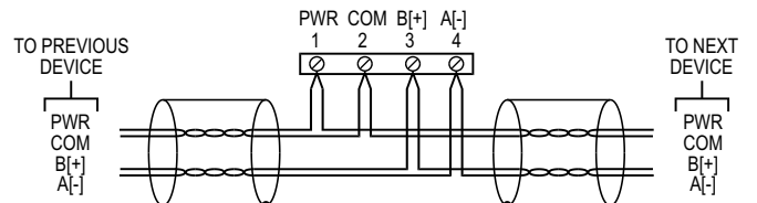
Figure 2: Common power supply wiring
