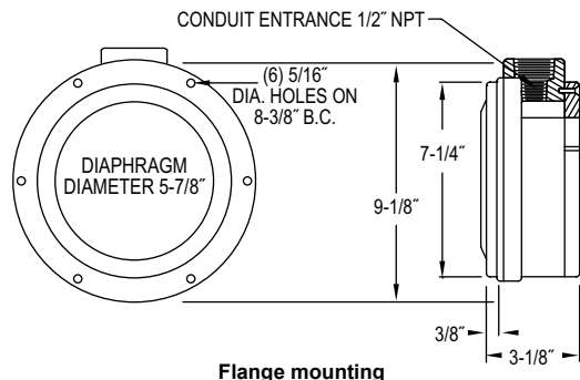
Flange mounting
